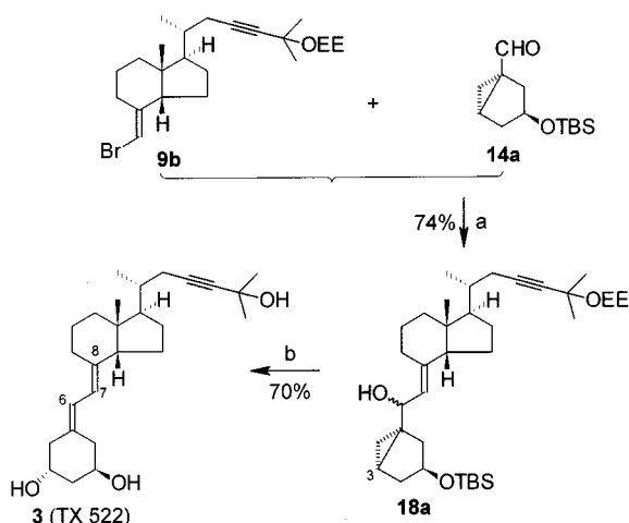
Scheme 5. (a) t BuLi, THF, -70 °C, 1 h; (b) PTSA, dioxane/H 2 O (1:1), 40–60 °C, 4 h
