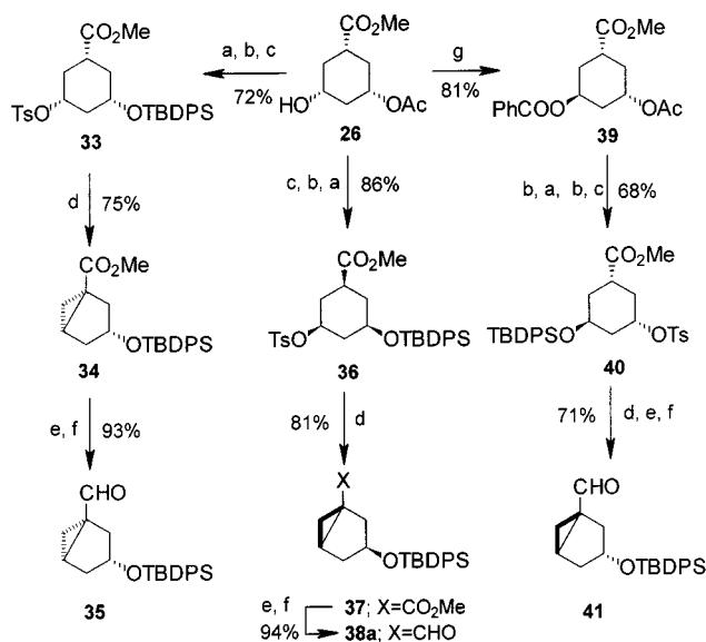
Scheme 3. (a) TsCl, Et 3 N, DMAP (cat.), CH 2 Cl 2 , room temp.; (b) K 2 CO 3 , MeOH, room temp.; (c) TBDPSCl, imidazole, DMF, room temp.; (d) t BuOK, t BuOH/THF, 55–60 °C; (e) DIBAL-H, CH 2 Cl 2 , –78 °C → –55 °C; (f) PCC, CH 2 Cl 2 , room temp., 1 h; (g) PhCO 2 H, DEAD, Ph 3 P, THF
