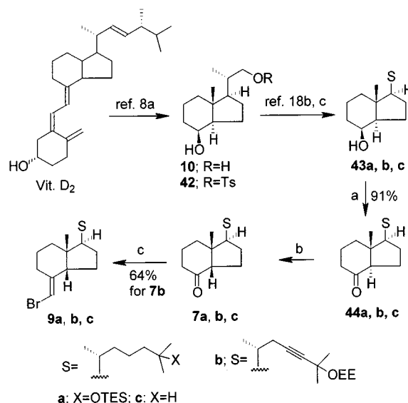
Scheme 4. (a) TPAP, NMO, 4 Å mol. sieves, CH 2 Cl 2 , room temp.; (b) NaOMe, MeOH, room temp., 24 h; (c) Ph 3 P + CH 2 Br.Br – , KHMDS, THF, –78 °C → room temp., 3 h; TES = triethylsilyl, EE = ethoxyethyl
